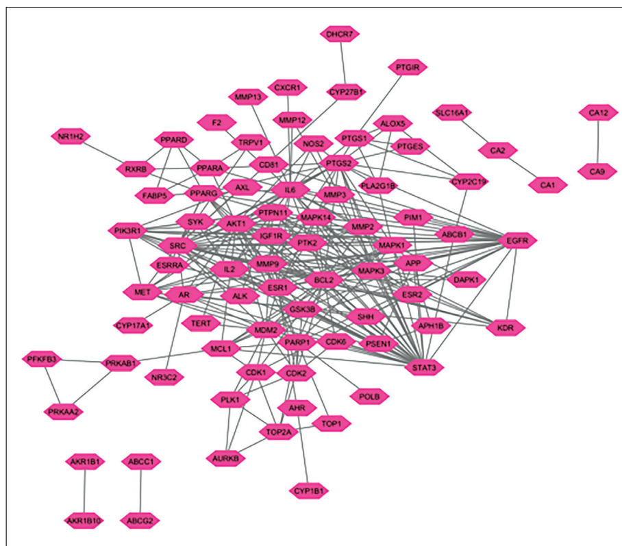
Figure 2. (a) PPI Visualized in Cytoscape.
