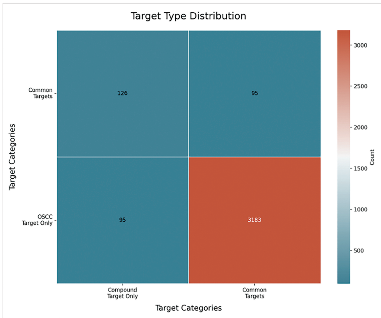
Figure 1. Heatmap Visualizing the Relationship Between Compound Targets and OSCC Targets.
