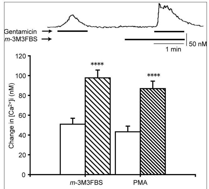
Figure 4: Enhancement of the gentamicin-induced [Ca^{2+}]_i elevation by m-3M3FBS and PMA. Gin-1 cells were stimulated with either gentamicin (500 \mu M) or gentamicin in combination with m-3M3FBS (20 \mu M) or PMA (20 \mu M). Upper panel: representative trace showing the effect of m-3M3FBS on the gentamicin-induced [Ca^{2+}]_i . Lower panel: effect of activators on the gentamicin-stimulated [Ca^{2+}]_i elevation. White columns represent the [Ca^{2+}]_i elevation stimulated by gentamicin alone; hatched bars denote gentamicin in combination with the activators. Data are mean \pm SEM, N = 32 (m-3M3FBS) or 22 (PMA). **** P < 0.001 compare to corresponding pretreated values
