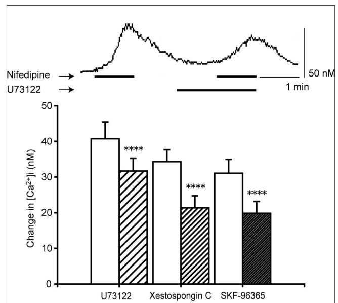
Figure 6: Inhibition of the nifedipine-induced [Ca^{2+}]_i elevation by pathway inhibitors. Cells were preincubated with U73122 (10 \mu M), xestospongine C (2 \mu M), or SKF-96365 (10 \mu M) prior to the application of nifedipine (10 \mu M). Upper panel: representative trace showing the effect of U73122 on the nifedipine-induced [Ca^{2+}]_i elevation. Lower panel: effect of nifedipine on [Ca^{2+}]_i in the absence (white bars) or presence (hatched bars) of inhibitors. Data are mean \pm SEM, N = 12 (U73122), 16 (xestospongine C), or 20 (SKF-96365). **** P < 0.001 compare to corresponding pretreated values
