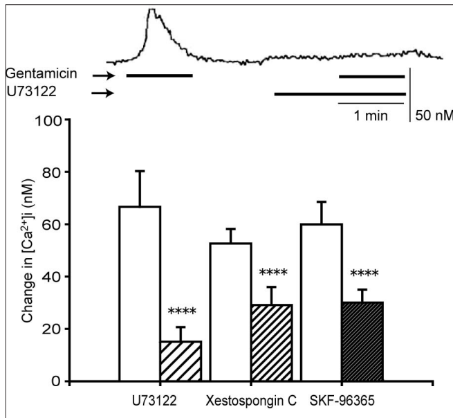
Figure 3: Effects of U73122, xestospongine C, and SKF-96365 on the gentamicin-induced [Ca^{2+}]_i elevation. Gentamicin (500 \mu M) was antagonized by U73122 (10 \mu M), xestospongine C (2 \mu M), and SKF-96365 (10 \mu M). The upper trace shows the effect of U73122 on the gentamicin-induced [Ca^{2+}]_i elevation. In the lower graph, white columns represent the [Ca^{2+}]_i elevated by gentamicin alone. Data are mean \pm SEM, N = 8 (U73122), 14 (xestospongine C), or 32 (SKF-96365). **** P < 0.001 compare to corresponding pretreated values
